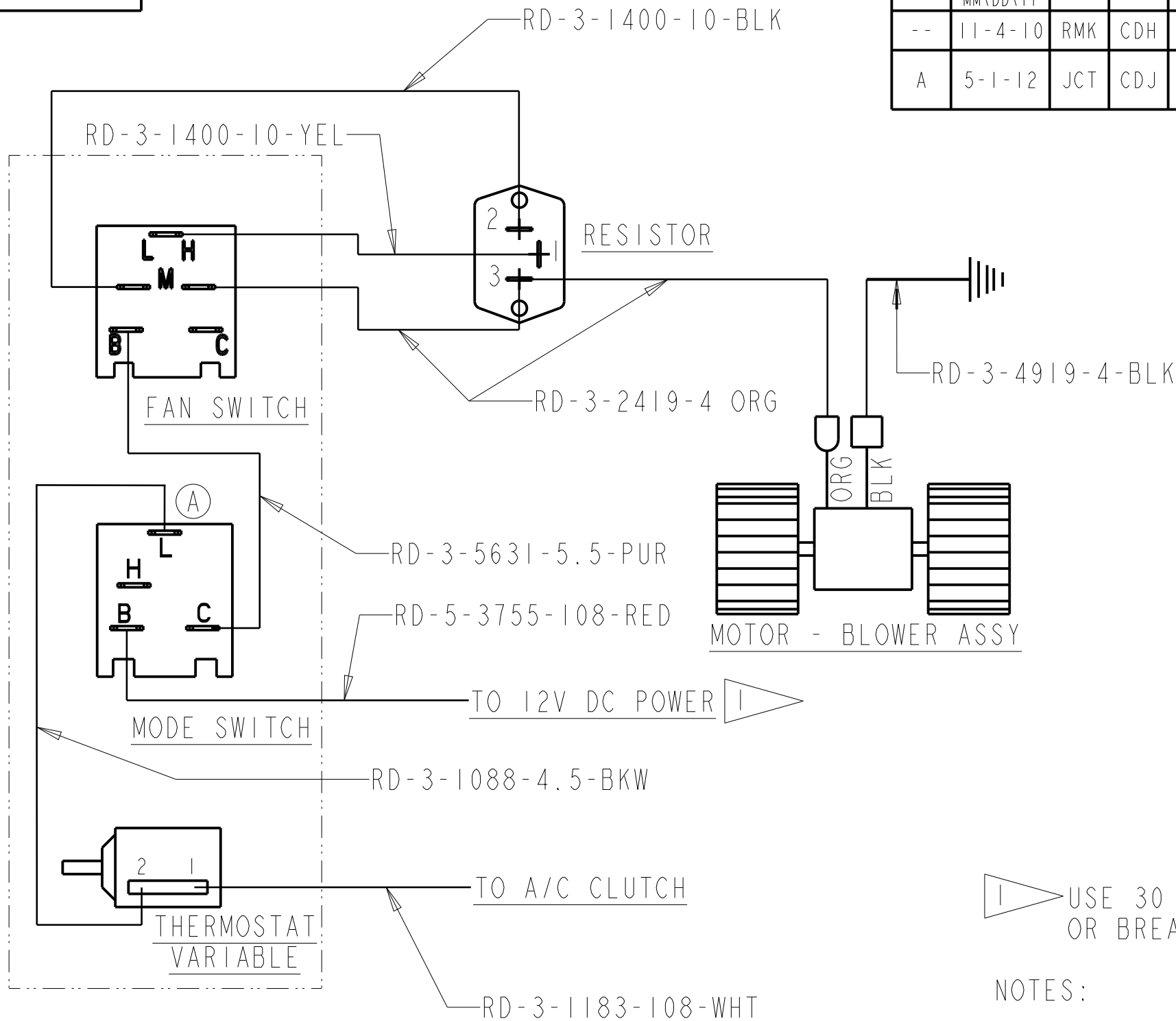
CONTROL PANEL (REAR VIEW)
