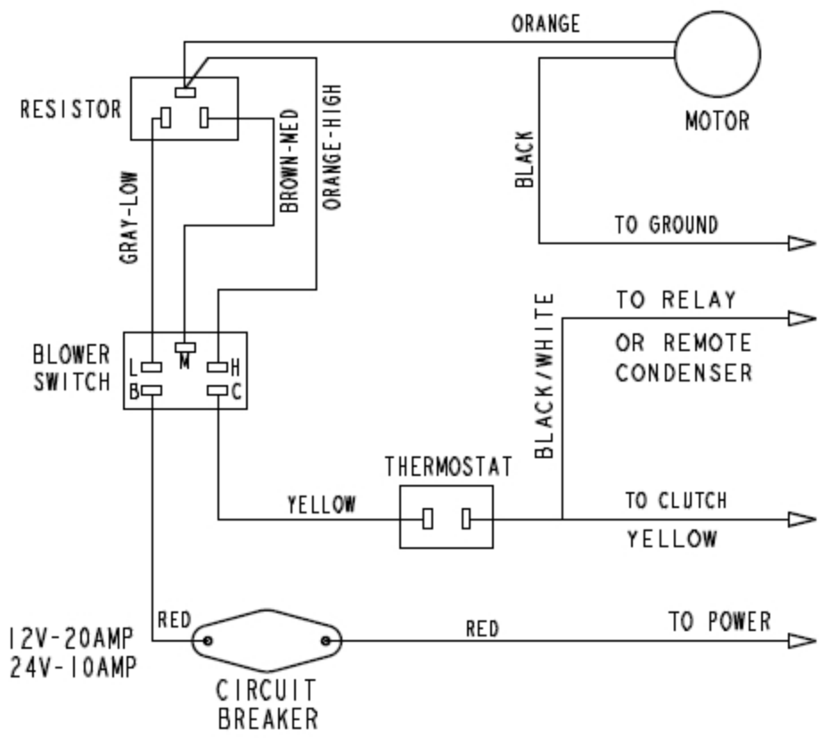
WIRING DIAGRAM - KK-600
