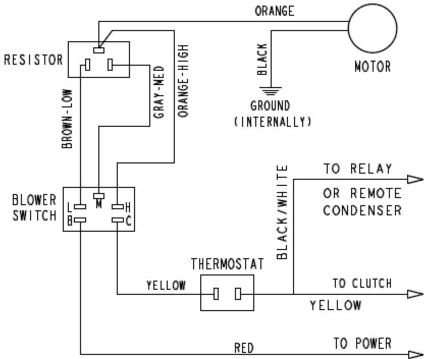
WIRING DIAGRAM
