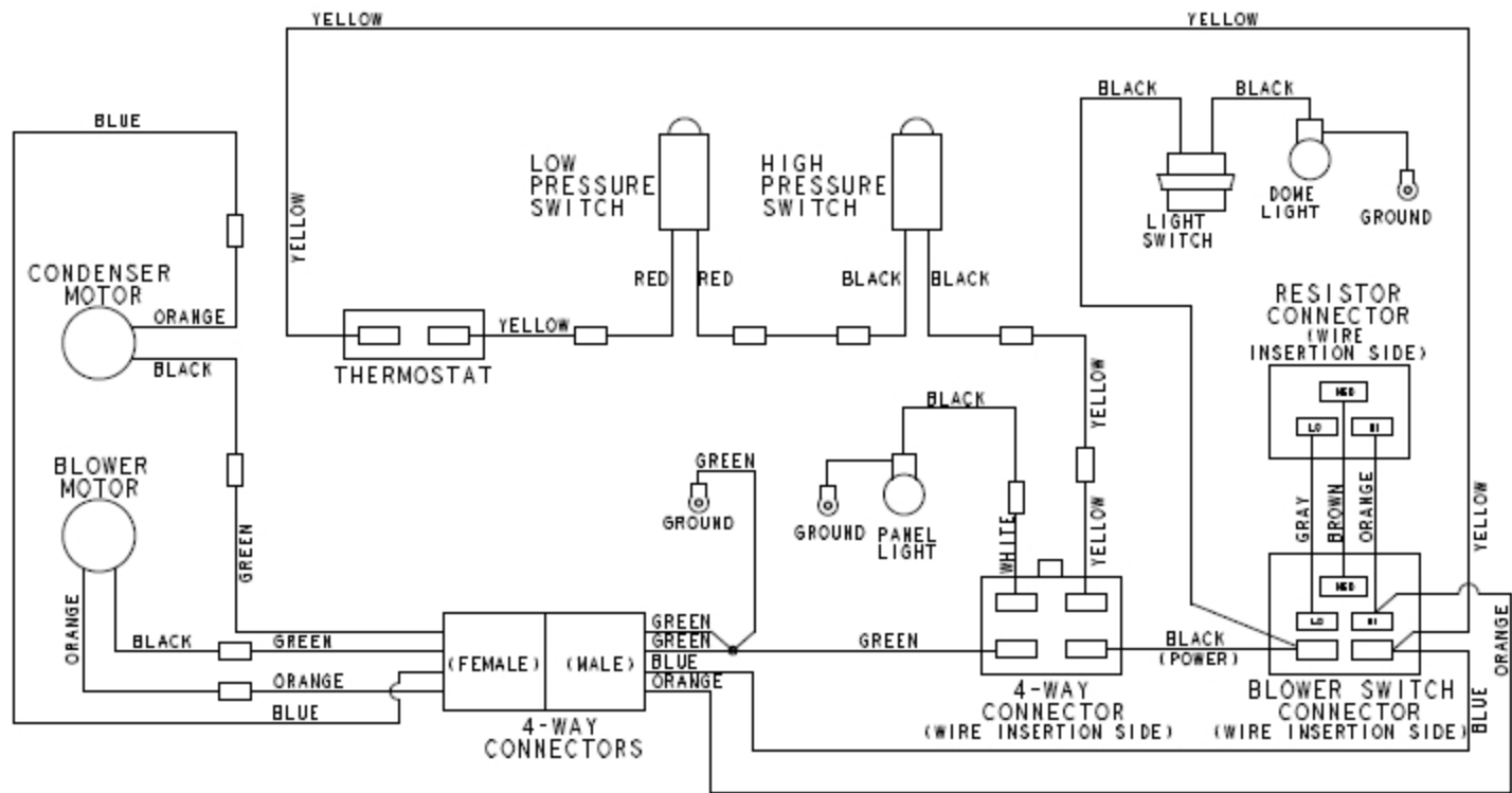
WIRING DIAGRAM - KA-300 AC (FOR NEGATIVE GROUND ONLY)
