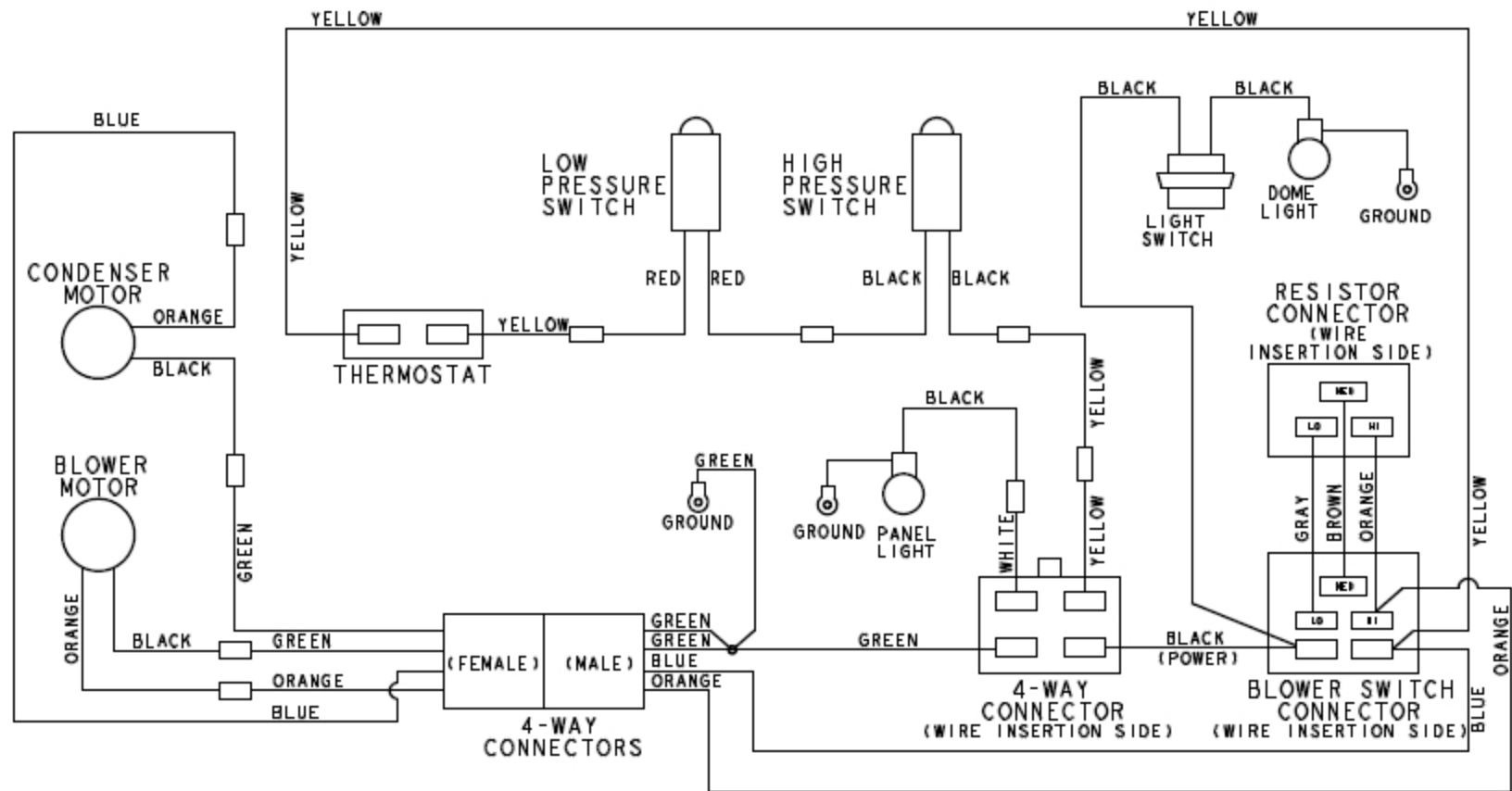
WIRING DIAGRAM - HD-1000 AC (FOR NEGATIVE GROUND ONLY)
