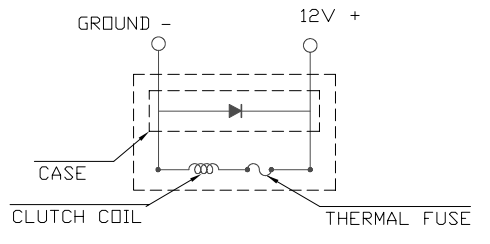
CIRCUIT DIAGRAM (FOR REFERENCE)
